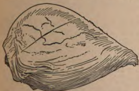
FIG. 118.—A pear-shaped lava projectile.
